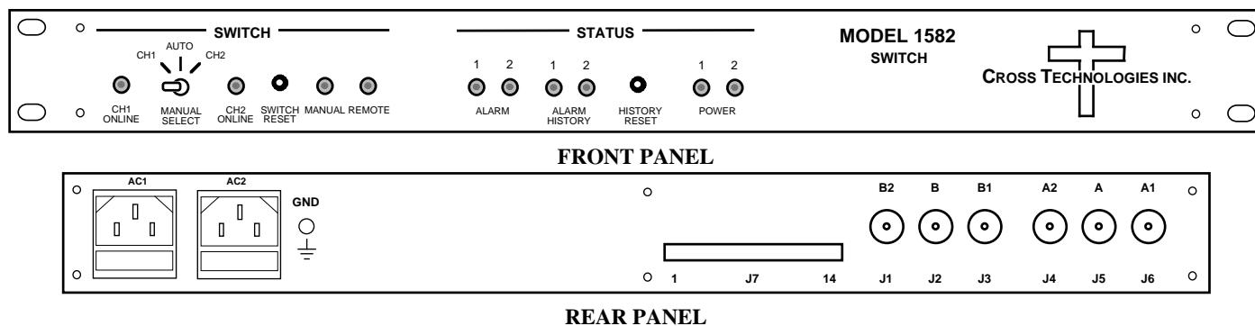
FIGURE 1.1 Model 1582-25L Front and Rear Panels
