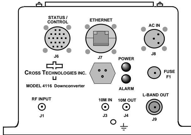
FIGURE 1.1 Model 4116-31-2831 Tri-Band Block Downconverter Front Panel
