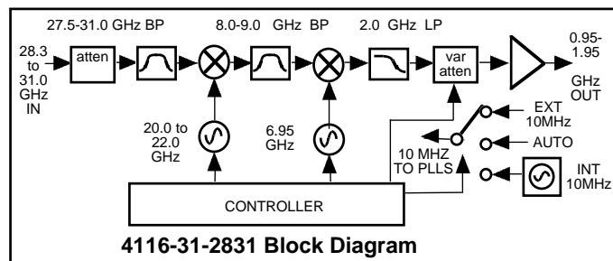
FIGURE 1. Model 4116-31-2831 Tri-Band Block Downconverter Block Diagram
