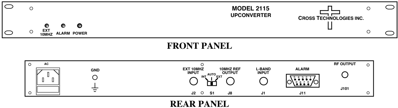
FIGURE 1.1 Model 2115-310-1600 Front & Rear Panels
