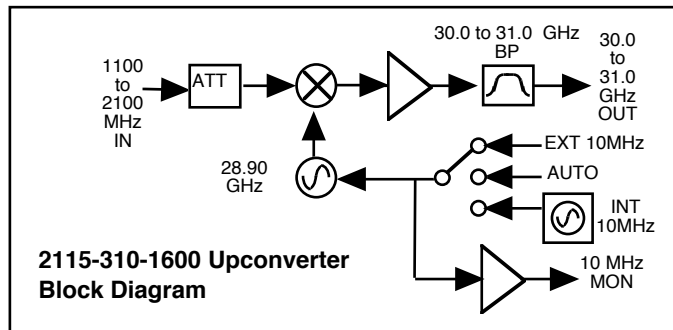
FIGURE 1.2 Model 2115-310-1600 Upconverter Block Diagram
