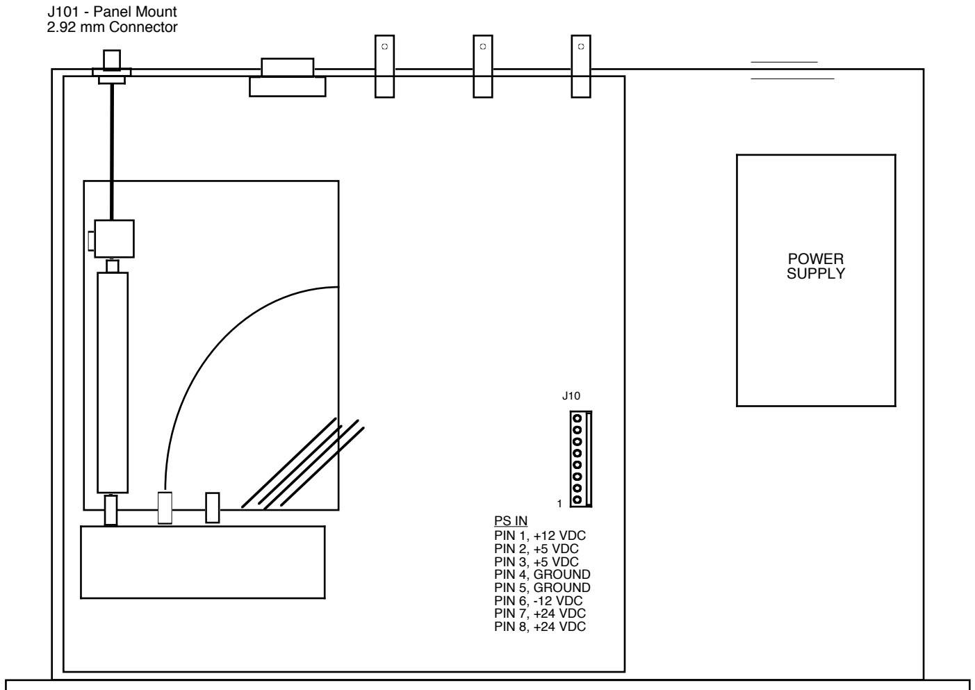
FIGURE 2.0 2115-310-1600 Mechanical Assembly
