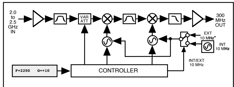
Block Diagram
